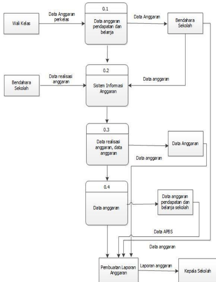
Gambar 3.2 Data Flow Diagram Level 0
